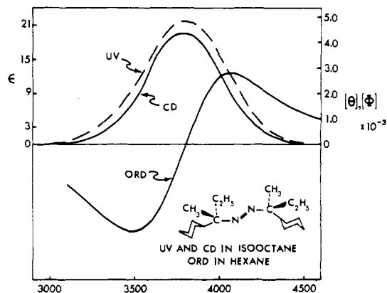
Figure 3. CD, ORD, and uv curves for trans -1,2-bis(2-cyclohexyl-2-butyl)diazene (1-C): CD, uv— isooctane ; ORD— hexane .
