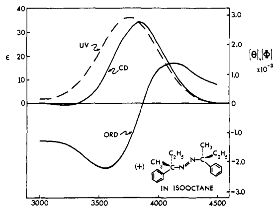
Figure 2. CD, ORD, and uv curves for trans -1,2-bis(2-phenyl-2-butyl)diazene (1-P) in isooctane. The short-wavelength portion of the CD curve with reversed sign has been confirmed as described in the text.
