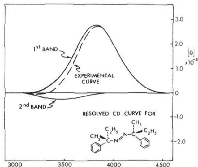
Figure 5. Circular dichroism curve for trans -1,2-bis(2-phenyl-2-butyl)diazene ( 1-P ) in isoctane and the two Gaussian components resolved from the experimental curve.
