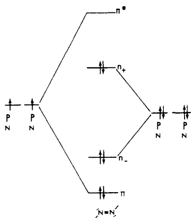
Figure 1. A qualitative energy level scheme for the combination arising from two nitrogen orbitals involved in formation of the diazene ( -N=N- ) group. The difference between the n_+ and n_- orbitals represents the splitting between the nonbonding nitrogen orbitals of the diazene group.
